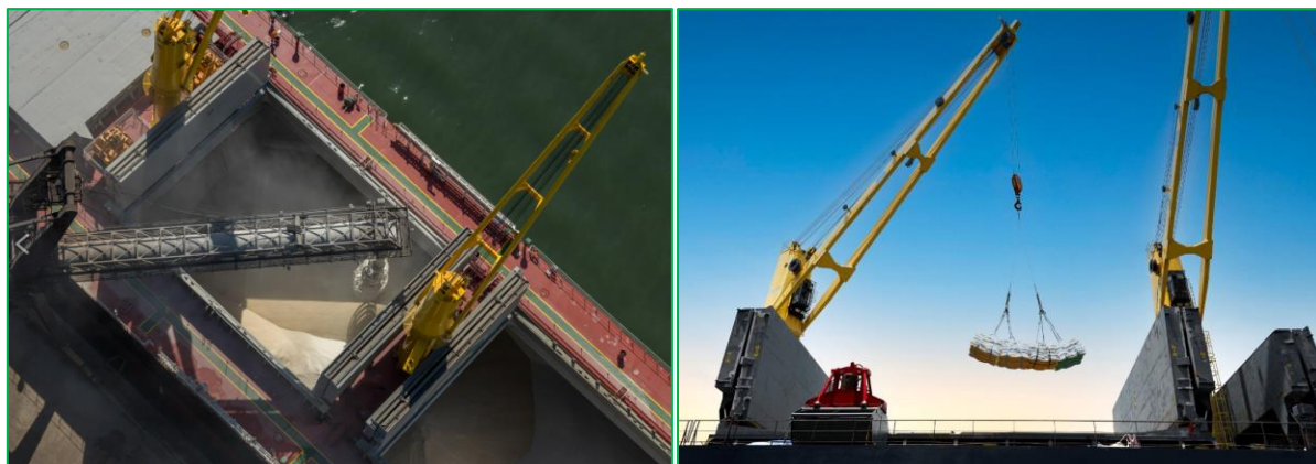
Pictures 6 &amp; 7: Loading sugar in bulk with shiploader (left) and bags with vessel's crane (right). Source: Copersucar/Shutterstock
